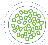
granulation
